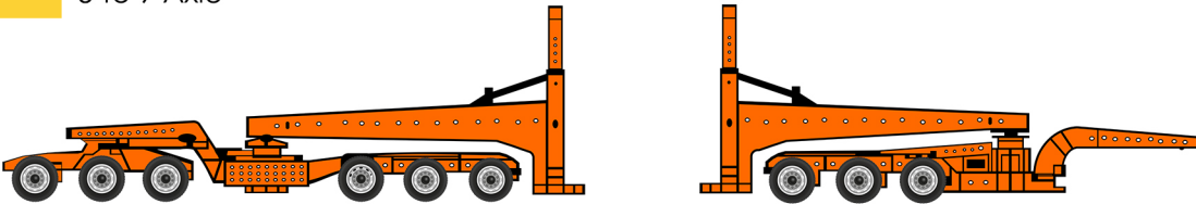
DOUBLE SCHNABLE WITH STEERABLE DOLLY 5 to 9 Axle
